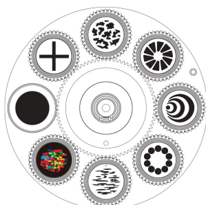
FOCUS SPOT 6Z GOBO WHEEL #2
