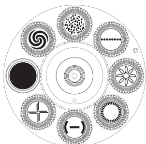
FOCUS SPOT 6Z GOBO WHEEL #1
